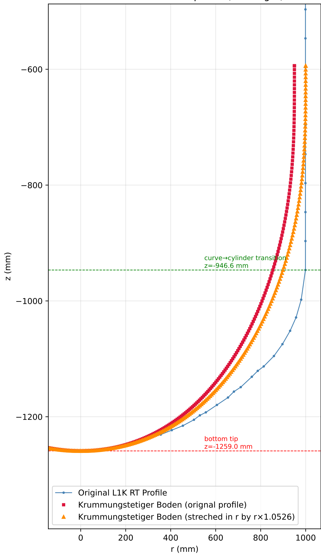
Reentrant tube: outer profile (full height)
